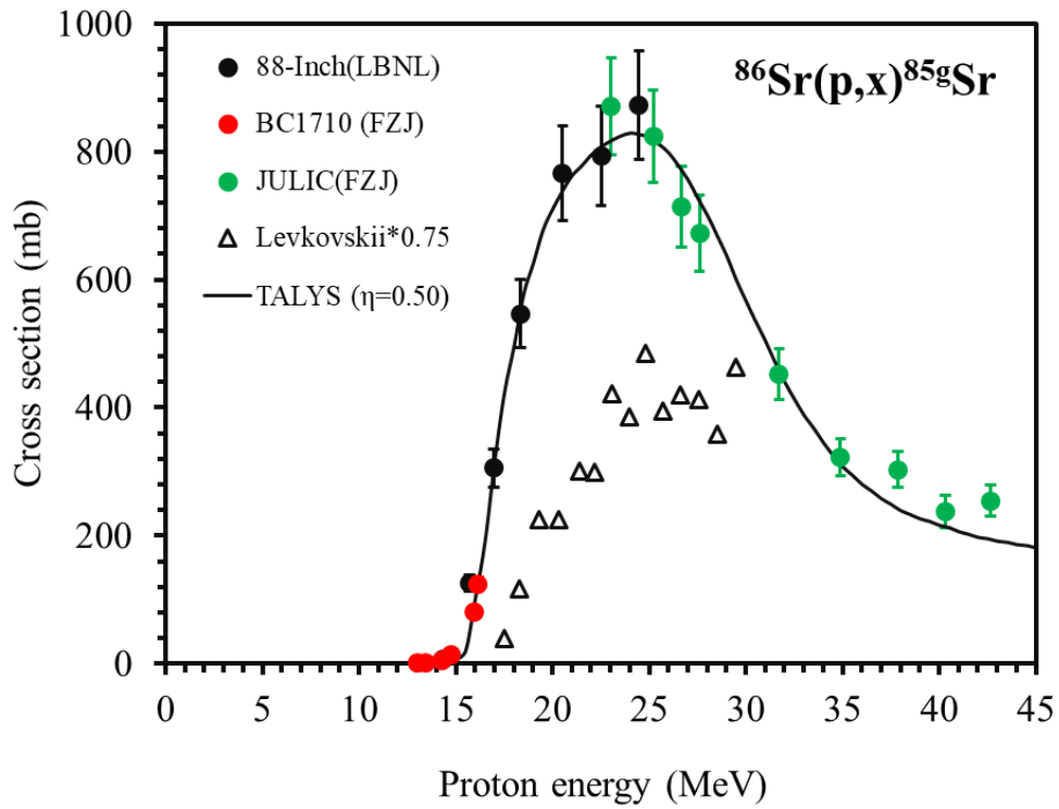
Fig. 4 Excitation function for the formation of the radionuclide ^{85g}\text{Sr} in proton irradiation of an enriched ^{86}\text{Sr} target. Our experimental data and the results of the model calculation represent cumulative cross sections.
