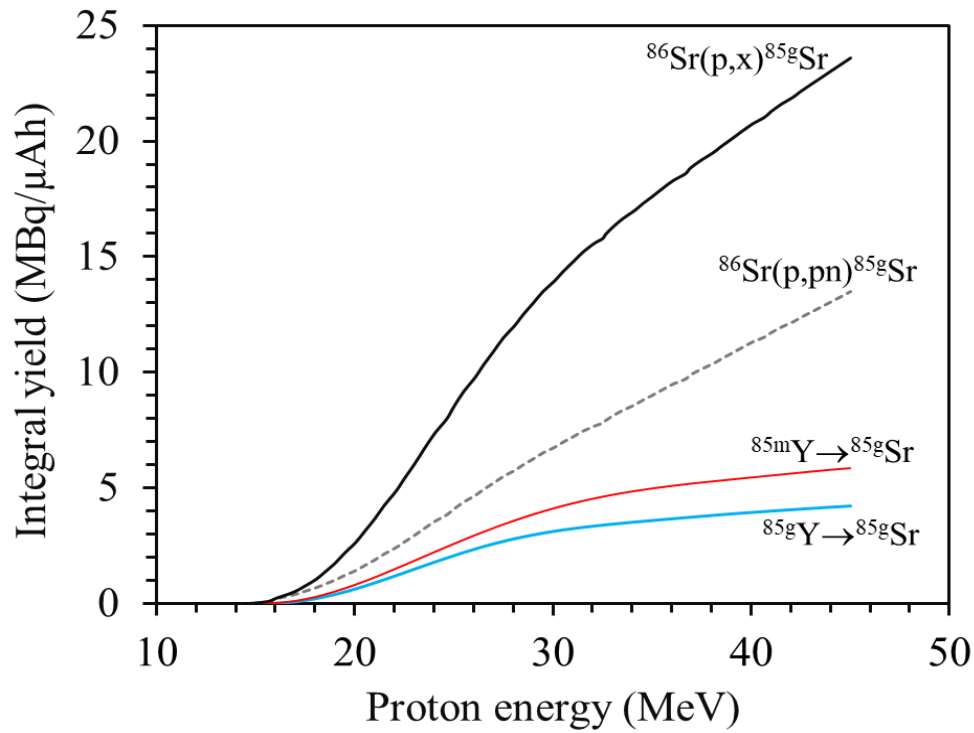
Fig. 6 Integral yield of the radionuclide ^{85g}\text{Sr} calculated from the measured excitation function of the ^{86}\text{Sr}(p,x) -process, assuming an irradiation time of 1 h at a proton beam current of 1 \mu\text{A} . The data are shown as a function of the proton energy. The yields of the three major contributing processes to the cumulative yield, i.e. the ^{86}\text{Sr}(p,pn) -reaction and the decay of the precursors ^{85g}\text{Y} and ^{85m}\text{Y} , are also shown.
