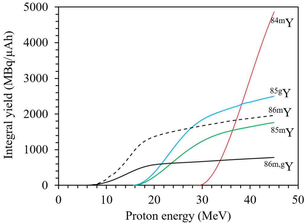
Fig. 5 Integral yields of the radionuclides ^{84m}, ^{85m}, ^{85g}, ^{86m}, ^{86m,g}\text{Y} calculated from the measured excitation functions of the ^{86}\text{Sr}(\text{p}, \text{x}) -processes, assuming an irradiation time of 1 h at a proton beam current of 1 \mu\text{A} . The data are shown as a function of the proton energy. The excitation function of ^{84m}\text{Y} was determined in this work; those other products were adopted from our earlier works [5, 6],
