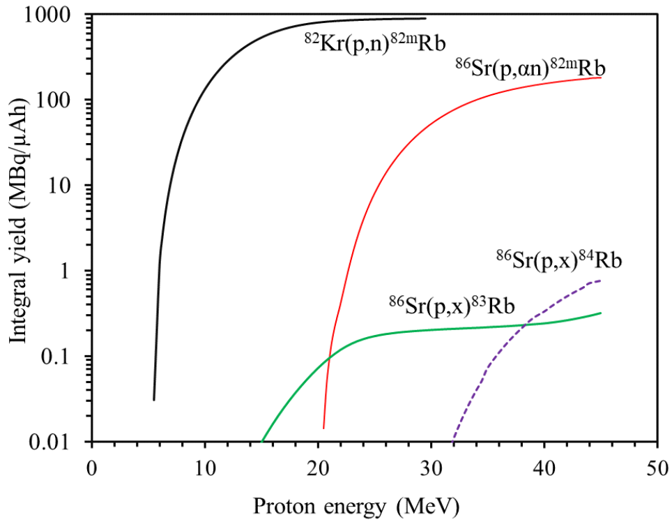
Fig. 7 Integral yields of the radionuclides ^{82m,83,84}\text{Rb} calculated from the measured excitation functions of the ^{86}\text{Sr}(\text{p},\text{x}) -processes, and the ^{82m}\text{Rb} yield also from the ^{82}\text{Kr}(\text{p},\text{n}) -process [11, 12], assuming an irradiation time of 1 h at a proton beam current of 1 \mu\text{A} . The data are shown as a function of the proton energy.
