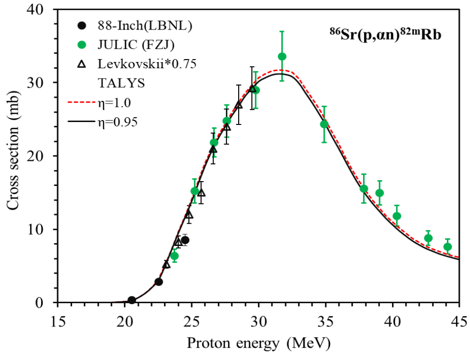
Fig. 3 Excitation function for the formation of the radionuclide ^{82m}\text{Rb} in proton irradiation of an enriched ^{86}\text{Sr} target. The calculated data are presented for two different \eta values.
