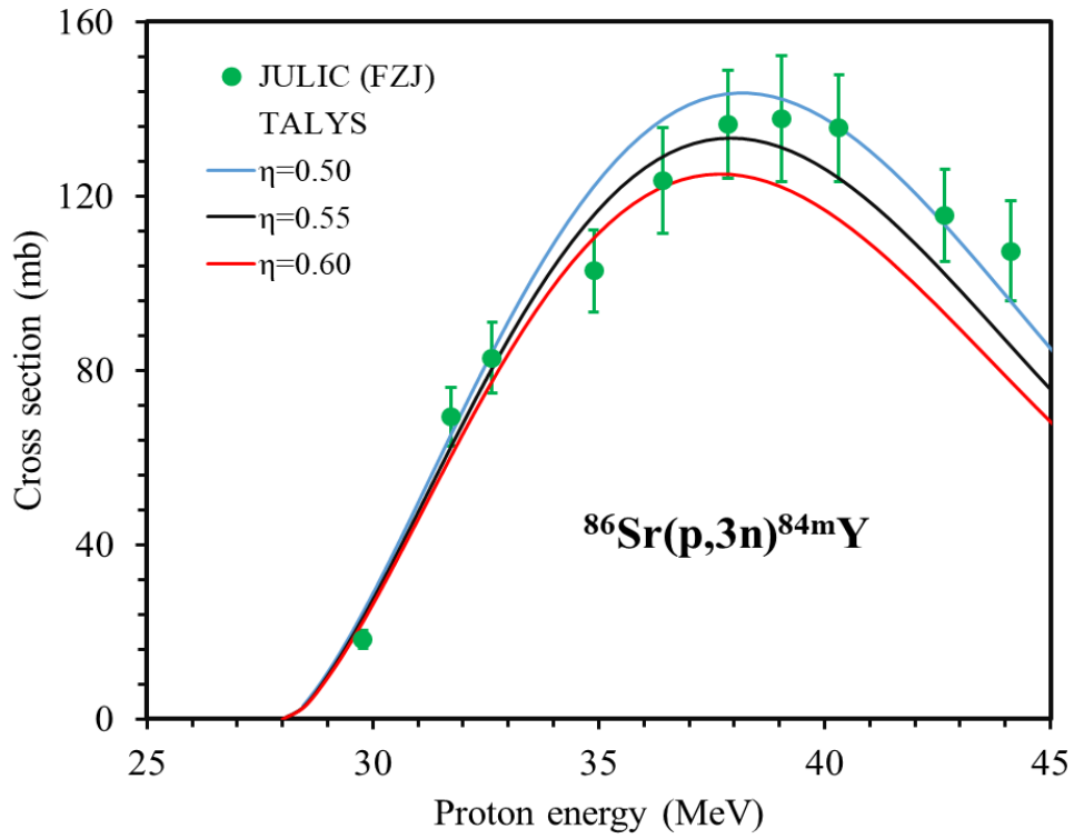
Fig. 2 Excitation function for the formation of the radionuclide ^{84m}\text{Y} in proton irradiation of an enriched ^{86}\text{Sr} target. The calculated data are presented for three different \eta values.
